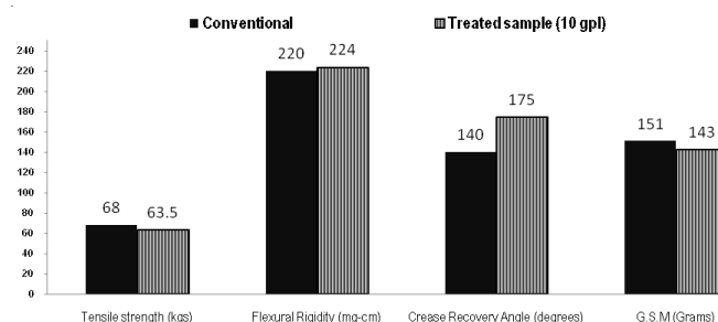
Figure 2. Physical properties of control and treated samples (treatment with 10 gpl concentration of PVAmHCl).
