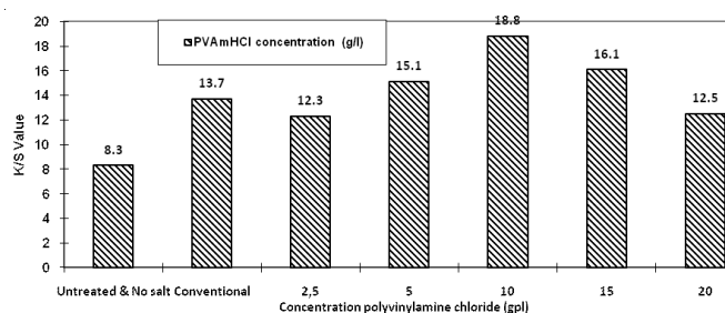
Figure 1. K/S value of control and treated samples.
